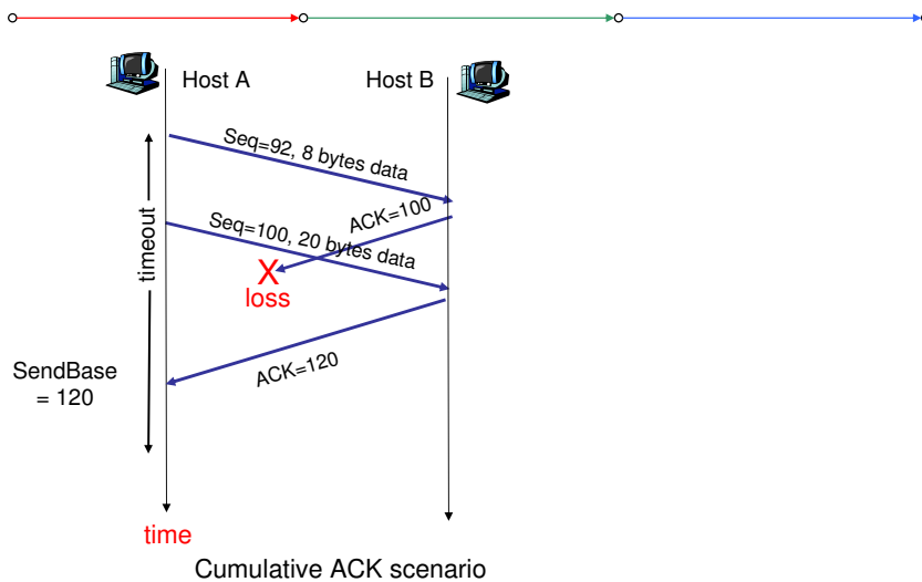
Cumulative ACK scenario
